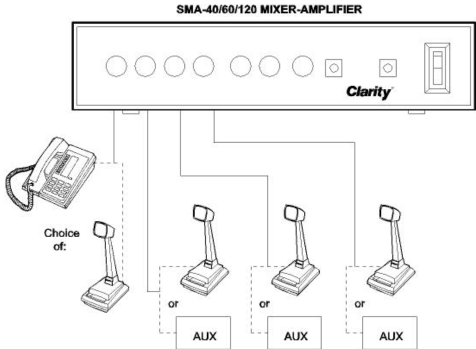
FIGURE 1 - TYPICAL INSTALLATION BLOCK DIAGRAM
