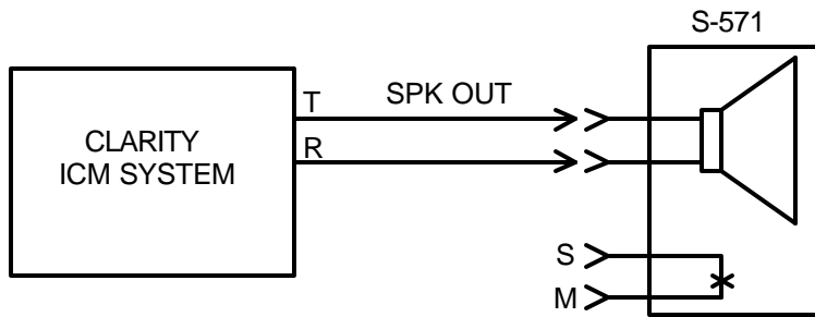
CONNECTIONS TO THE S-571
